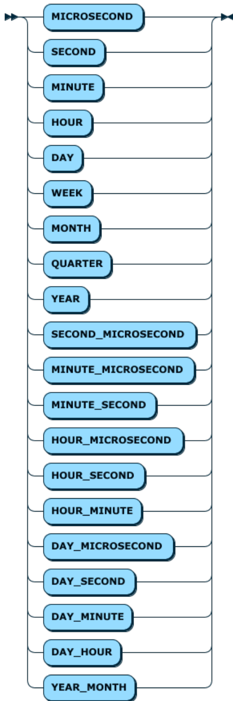
Figure 12.20 INTERVAL_UNIT
