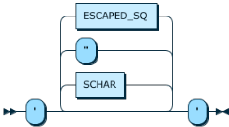
Figure 12.40 STRING_SQ
