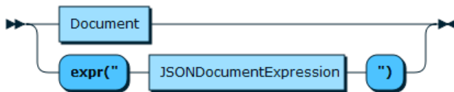
Figure 11.41 DocumentOrJSON
