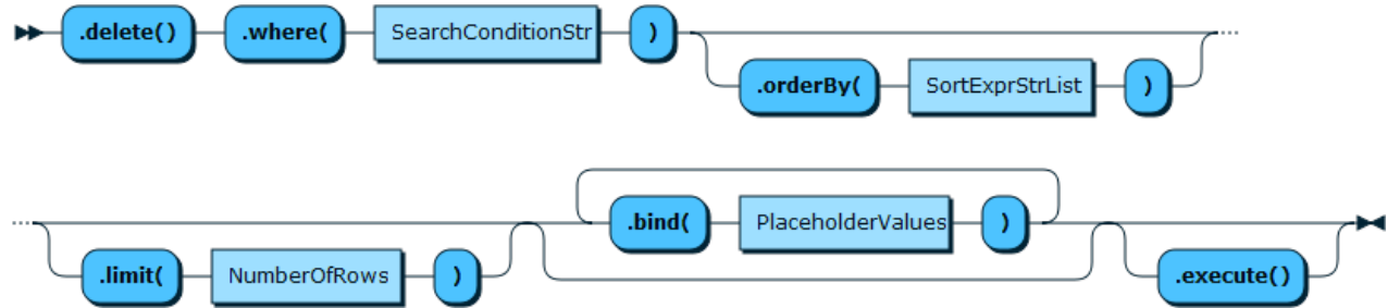
Figure 6.4 Table.delete() Syntax Diagram
