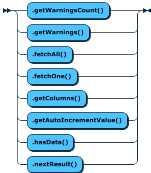
Figure 11.23 SqlResult
