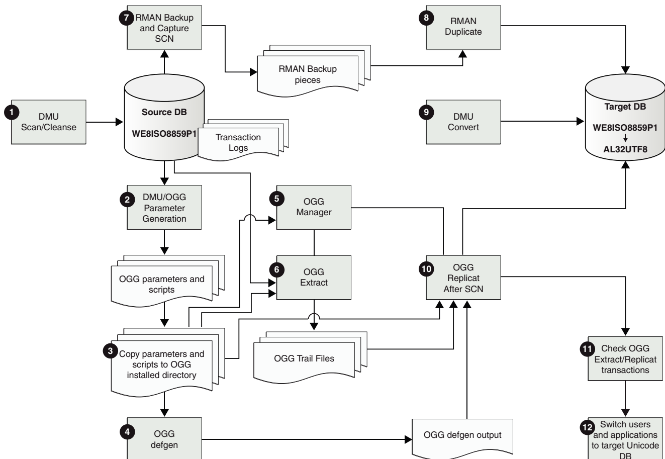
Figure 5-1 Steps for Migrating Oracle Database to Unicode in Near-Zero Downtime
