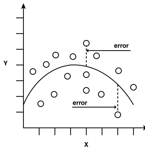
Figure 7-6 Nonlinear Regression With a Single Predictor
