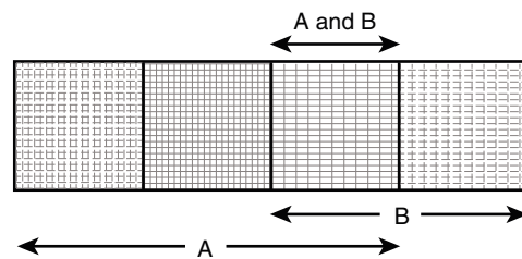
Figure 7-11 Conditional Probabilities in Bayes' Theorem
