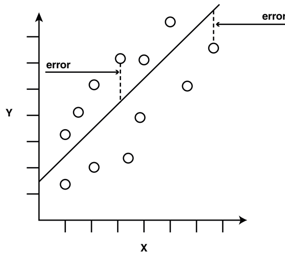
Figure 7-5 Linear Regression With a Single Predictor
