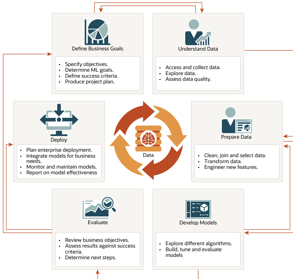
Figure 1-3 Machine Learning Process Workflow
