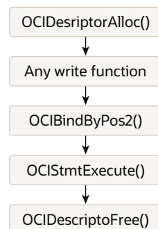
Figure 22-2 Calling Sequence for Writing JSON Data
