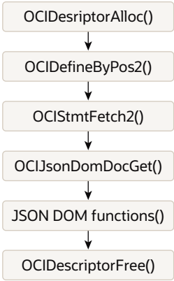
Figure 22-3 Calling Sequence for Reading JSON Data
