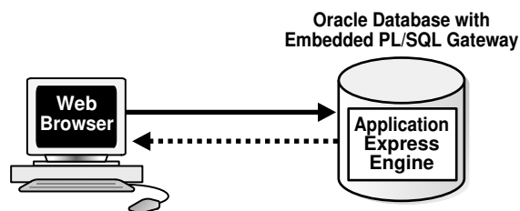
Figure 23-1 APEX with Embedded PL/SQL Gateway
