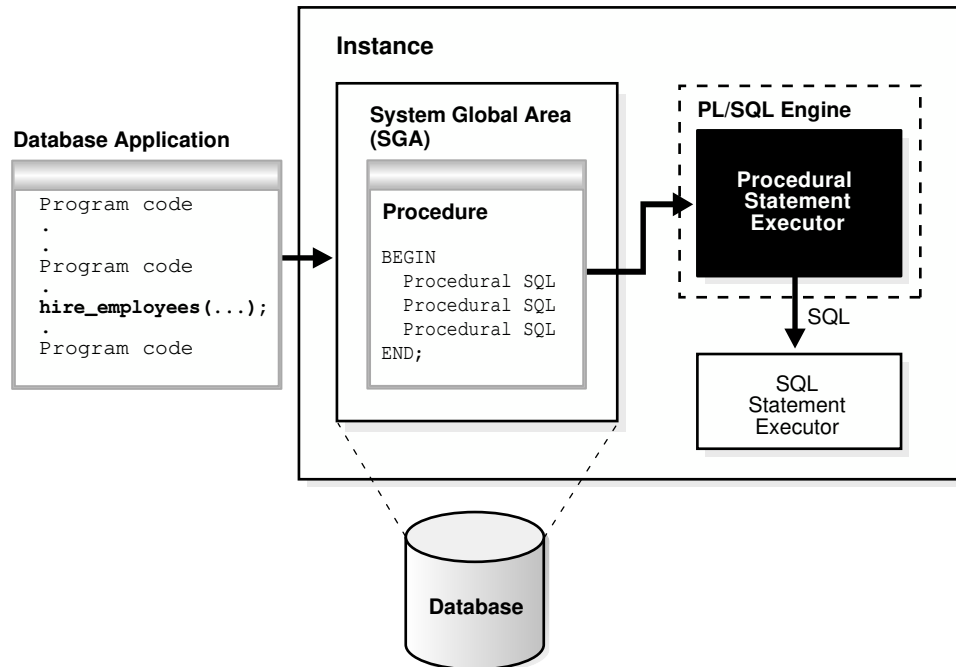
Figure 11-3 The PL/SQL Engine and Oracle AI Database
