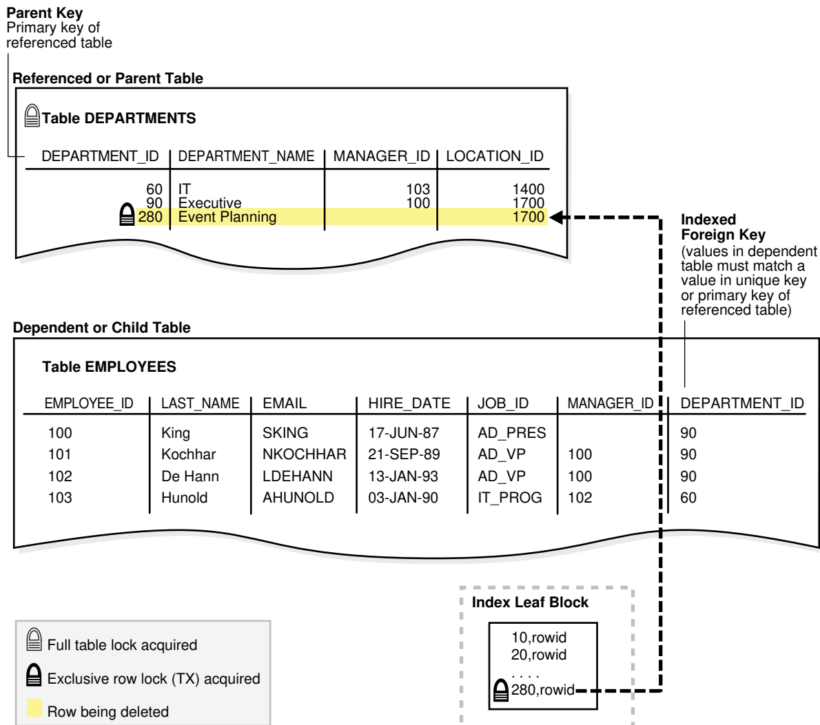
Figure 12-4 Locking Mechanisms with Indexed Foreign Key
