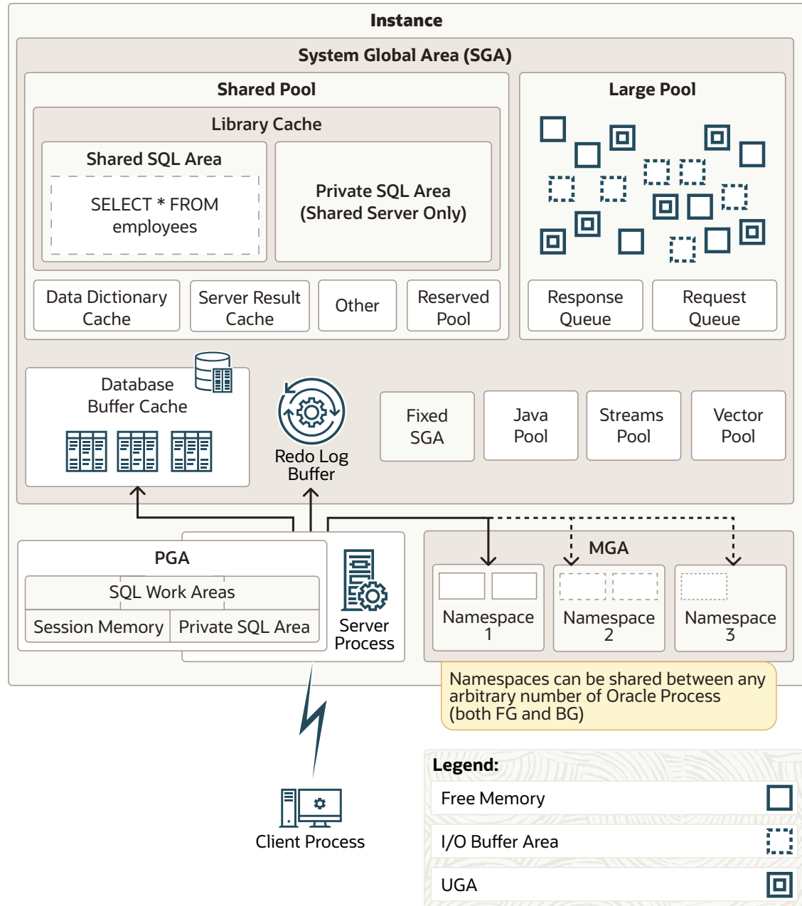
Figure 17-1 Oracle AI Database Memory Structures
