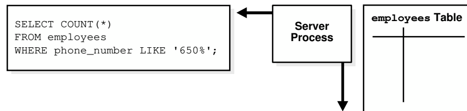
Figure 18-5 Serial Full Table Scan
