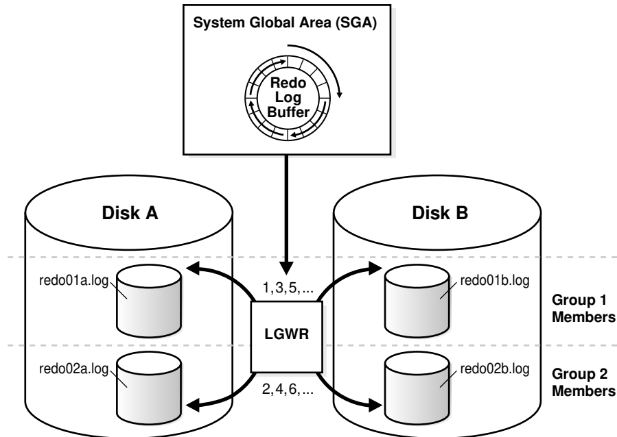
Figure 14-8 Multiple Copies of Online Redo Log Files
