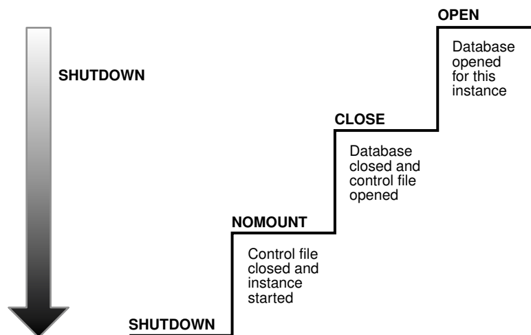
Figure 16-4 Instance and Database Shutdown Sequence
