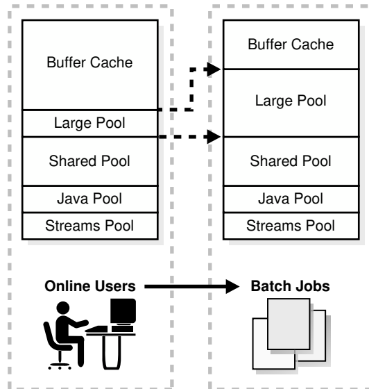
Figure 22-6 Automatic Memory Management
