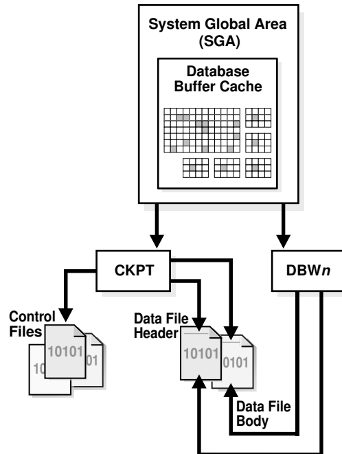
Figure 18-4 Checkpoint Process
