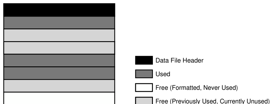
Figure 14-6 Space in a Data File
