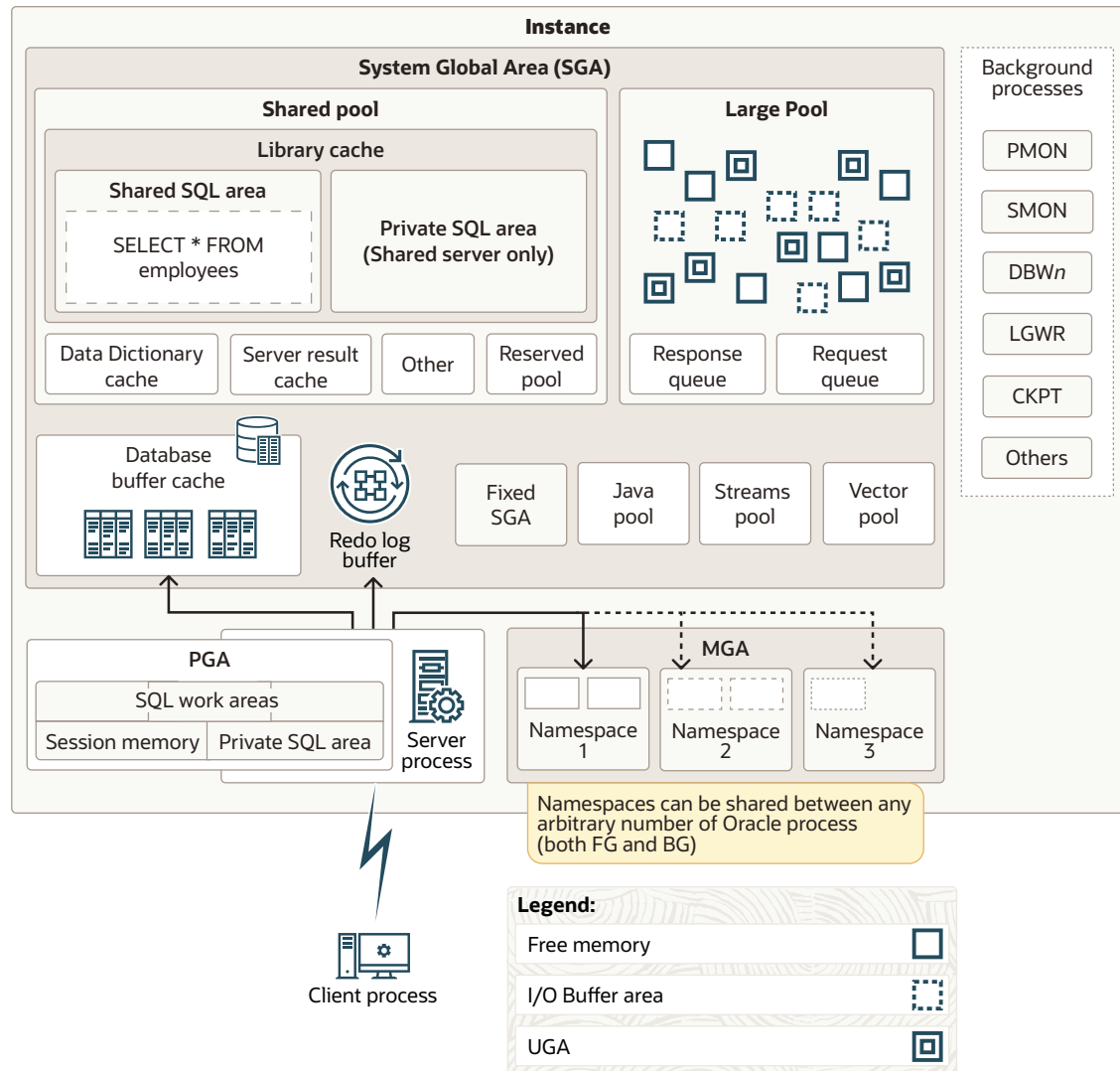
Figure 16-1 Database Instance
