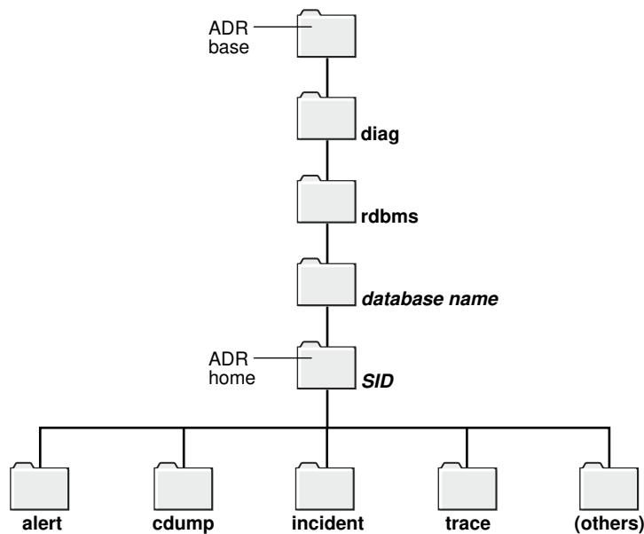
Figure 16-8 ADR Directory Structure for an Oracle AI Database Instance
