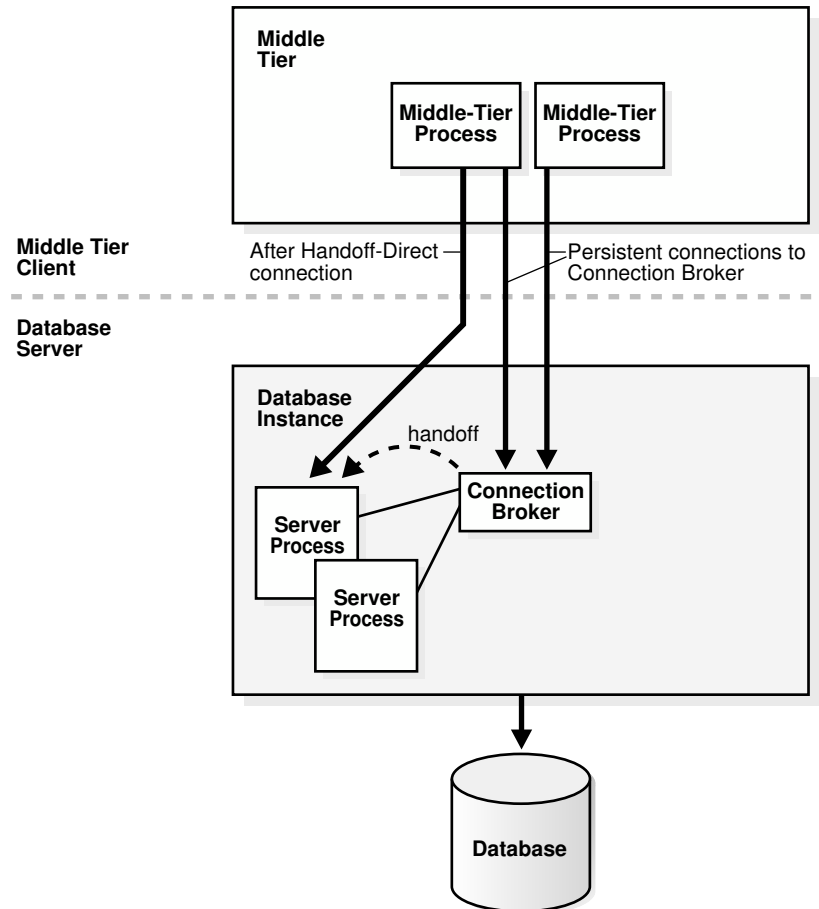
Figure 19-10 DRCP
