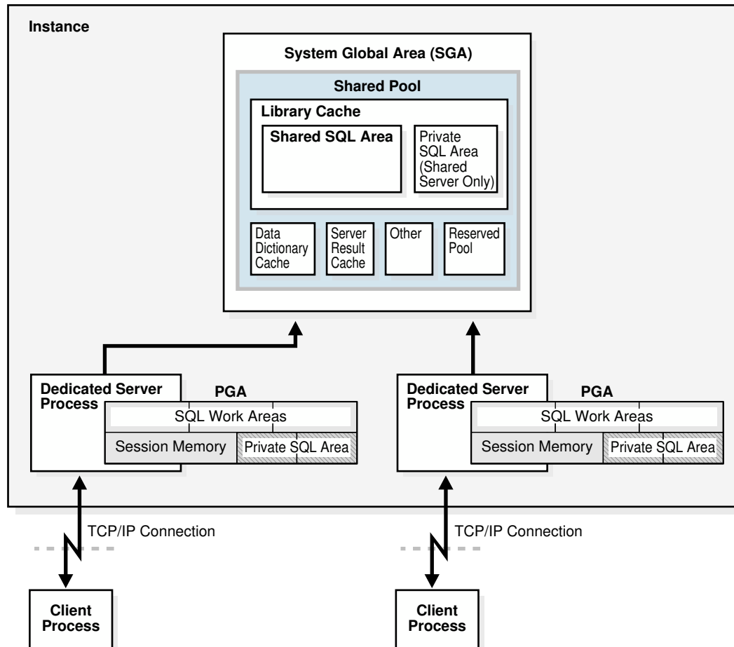
Figure 19-8 Oracle AI Database Using Dedicated Server Processes
