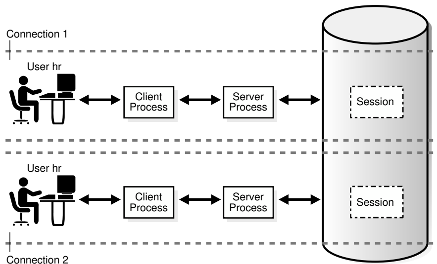
Figure 18-2 One Session for Each Connection
