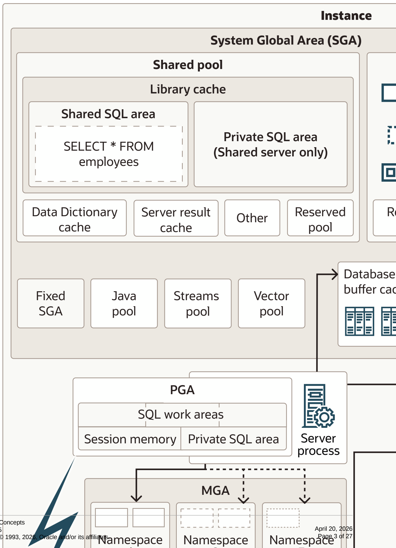
Figure 18-1 Oracle Processes and the SGA
