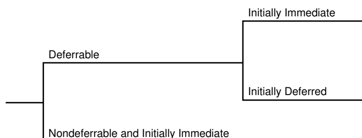
Figure 7-3 Options for Deferrable Constraints and Assertions
