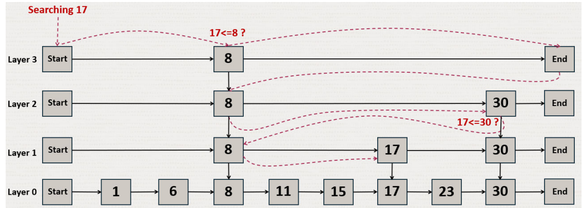
Figure 21-3 Probability Skip List Structure
