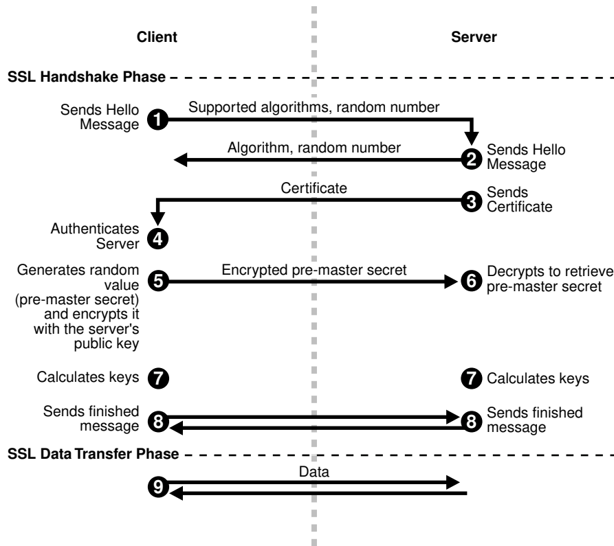
Figure 6-1 SSL Handshake
