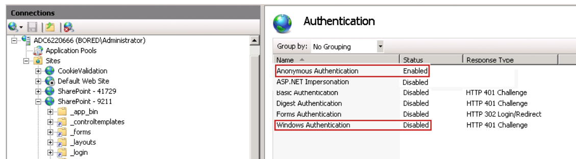
Figure 51-4 Impersonation Authentication
