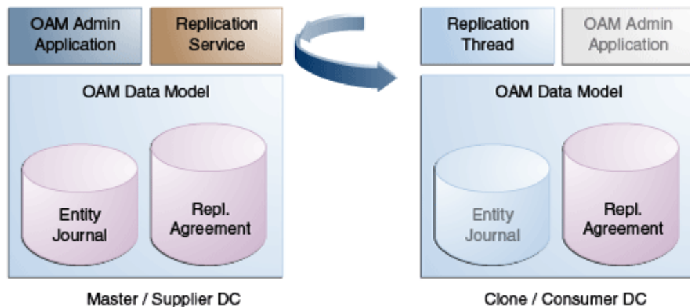
Figure 19-1 Replication Flow
