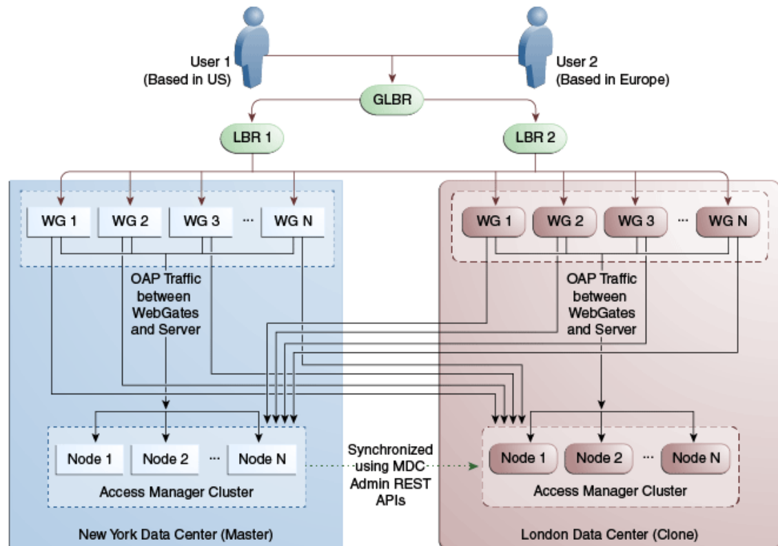
Figure 17-9 Active-Active Topology
