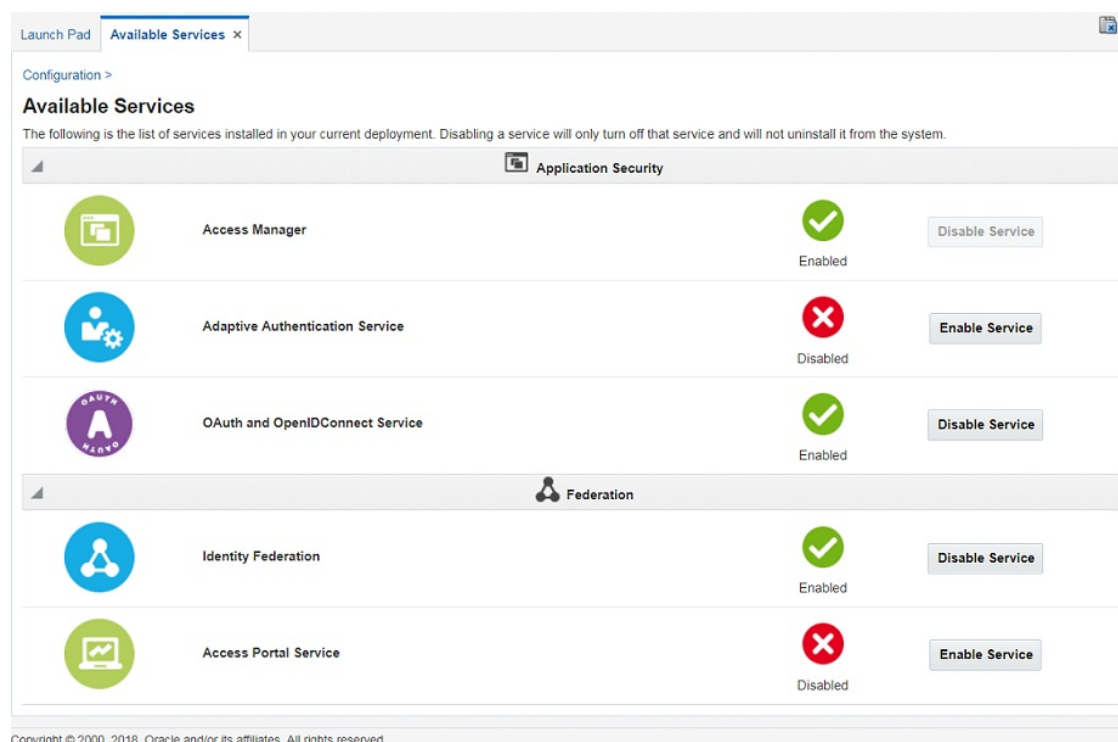
Figure 3-2 Available Services
