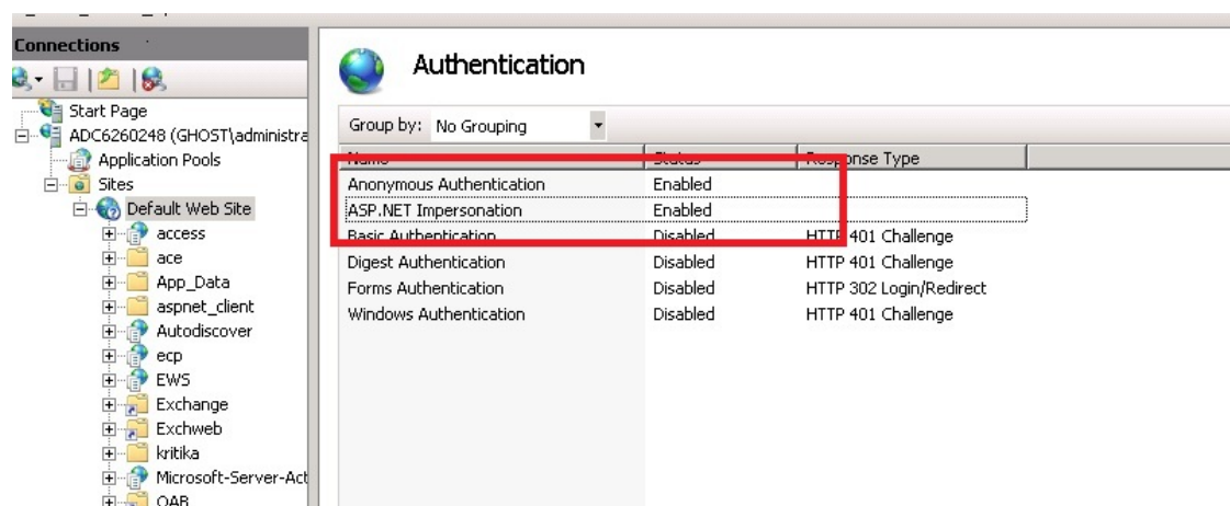
Figure 52-4 Impersonation Authentication
