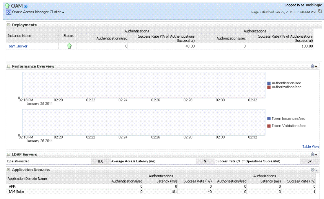
Figure 12-8 Cluster Page
