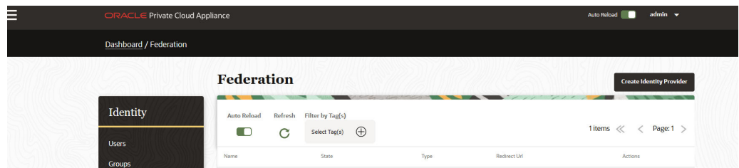
Figure 54-3 Create IDP
