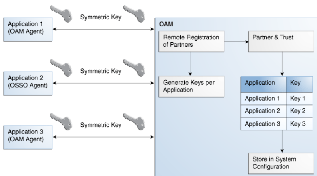
Figure 15-5 Key Generation
