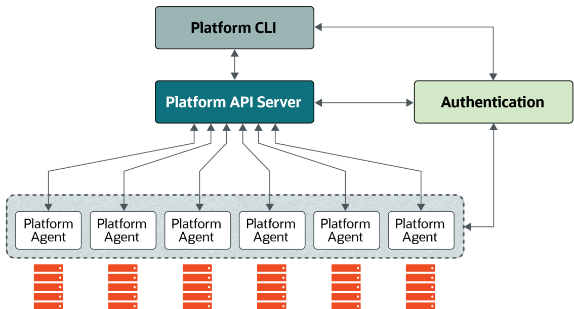
Figure 3-1 Architecture
